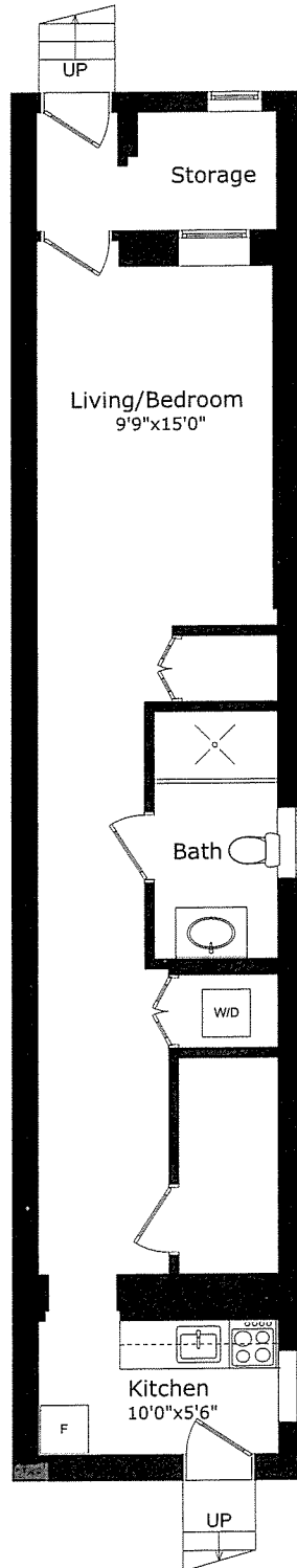
LOWER FLOOR
