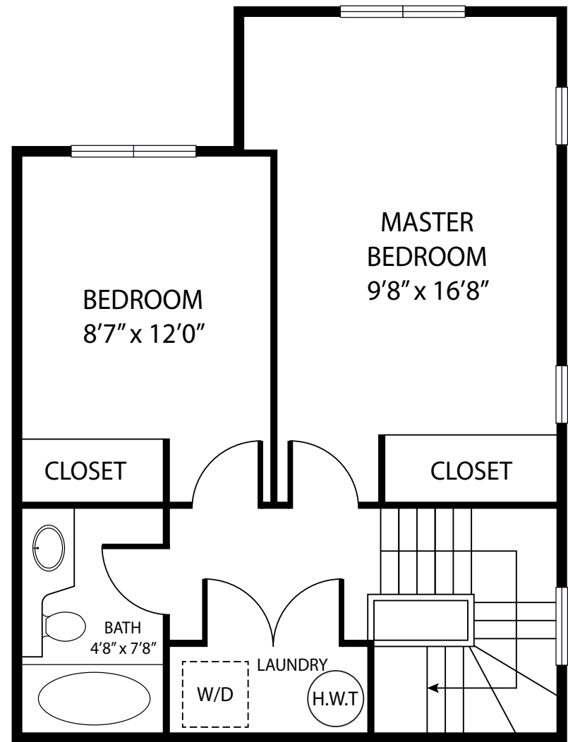
UPPER LEVEL 470 SQ.FT
